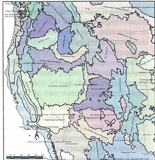
Level III Ecoregions of the Western US
